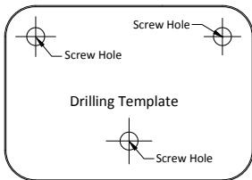
Figure 3-2 Drill Template
