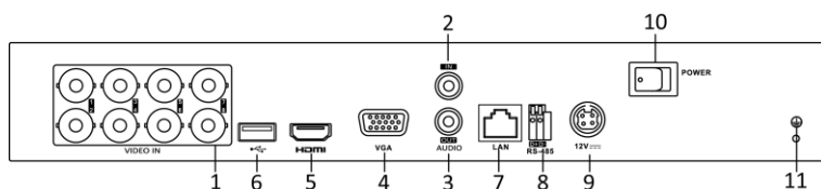
Figure 1. 6 Rear Panel of 720P Series
